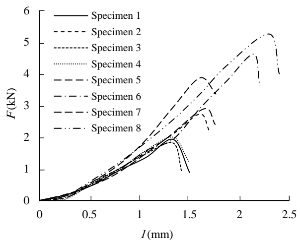
Fig. 5 Load-displacement diagram of specimens (average of three specimens)
