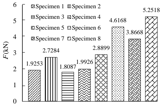
Fig. 6 Shear strength of the specimens (average of three specimens)
