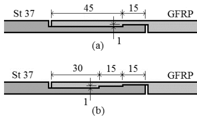
Fig. 2 Schematic of the stepped specimens geometry, a) with one reverse step, b) with two reverse steps (dimensions in millimeters)
