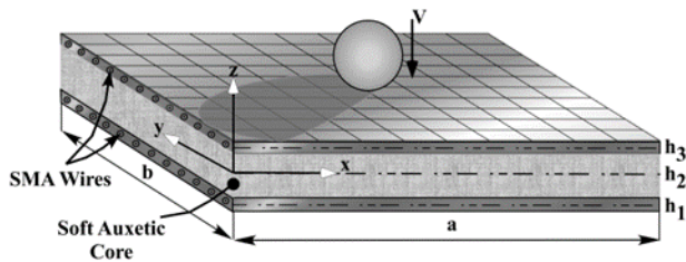
Fig. 1 The geometric parameters of the composite sandwich plate with embedded SMA wires and soft core and the indenter
