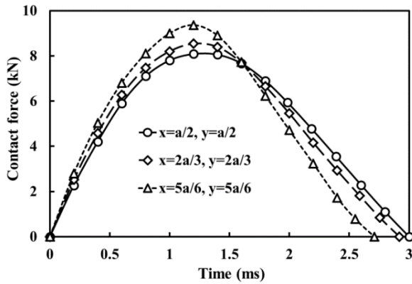
Fig. 22 Influence of the eccentricity of the impact on time history of the contact force of the composite sandwich plate reinforced by SMA wires with auxetic core
