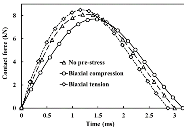
Fig. 24 Effects of various types of in-plane biaxial preloads on time history of the contact force of composite sandwich plate reinforced by SMA wires with auxetic core
