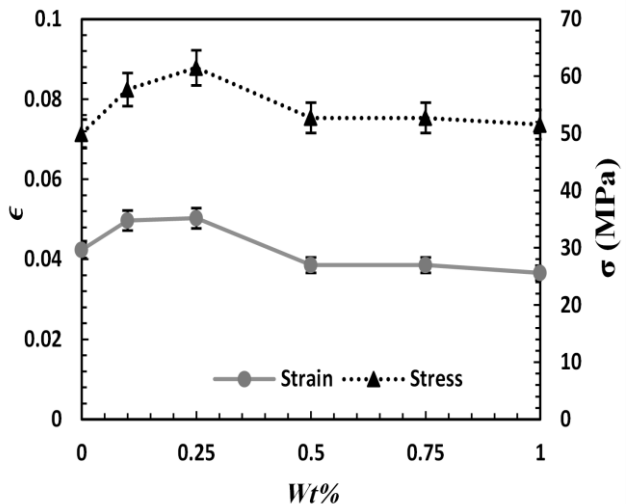
Fig. 4 Ultimate stress and strain for 6 percent weight of nanocomposite
