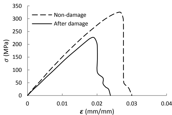
Fig. 5 Results of bending test for control sample in two states non-damage and after damage
