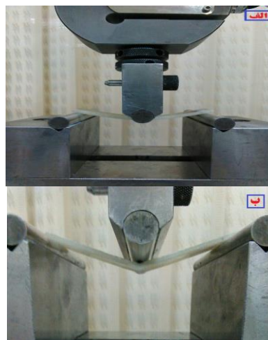
Fig. 4 Three-point bending test, s procedure, a) at the moment and b) at the end of test until sampel, s fracture
