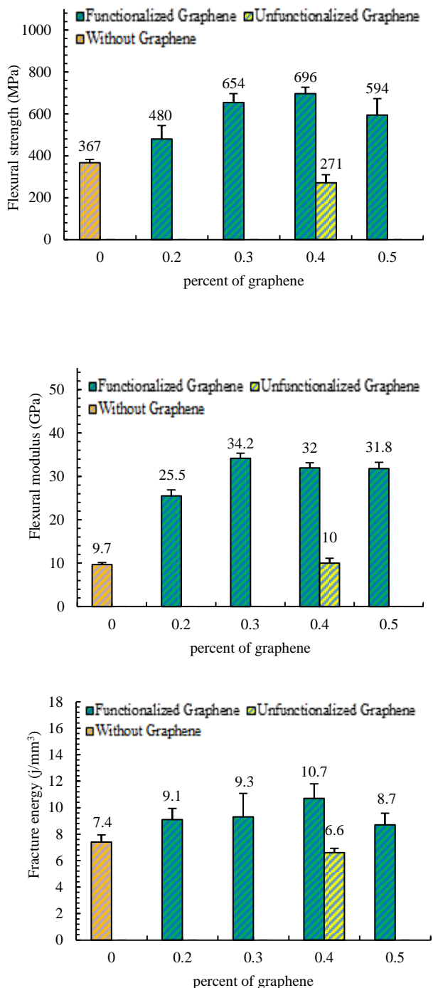
Fig. 5 The effect of graphene on the flexural properties of basalt fibers/ epoxy nanocomposites. a) Flexural strength, b) Flexural modulus and c) Fracture energy
