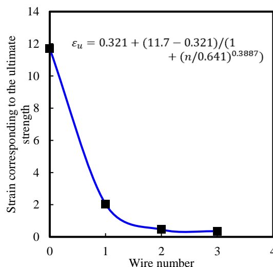
Fig. 12 The curve fitting related to the strain values corresponding to the ultimate strength of pure latex samples
